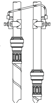
Diagram of earth continuity connections
